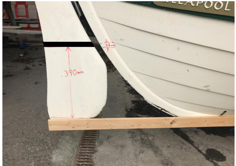
Reference water line 390mm above keel rabbet
